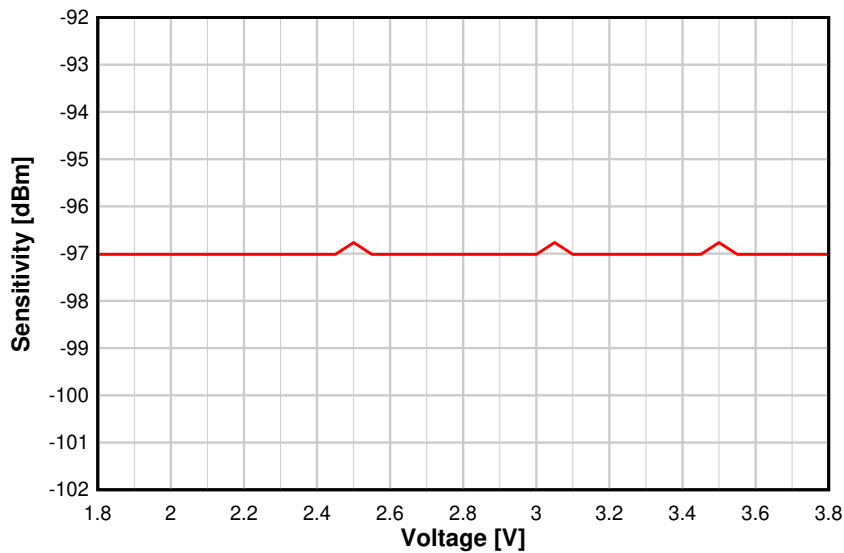
Figure 5-16. Sensitivity vs. Supply Voltage (VDDS) (BLE 1 Mbps, 2.44 GHz, DCDC Off)
