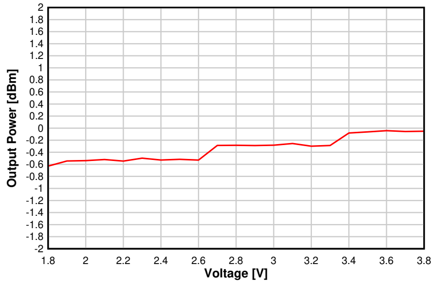
Figure 5-20. Output Power vs. Supply Voltage (VDD5) (BLE 1 Mbps, 2.44 GHz, 0 dBm)
