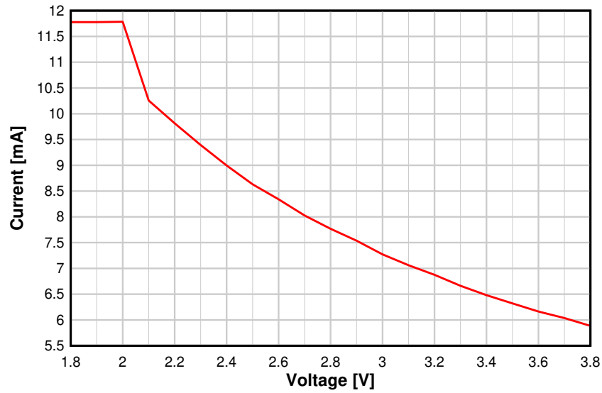
Figure 5-8. RX Current vs. Supply Voltage (VDD5) (BLE 1 Mbps, 2.44 GHz)
