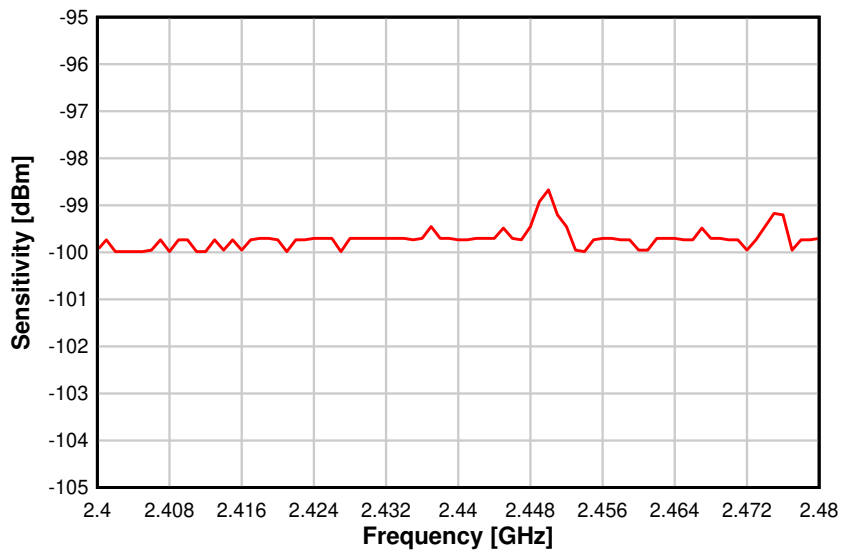
Figure 5-12. Sensitivity vs. Frequency IEEE 802.15.4 (OQPSK DSSS1:8, 250 kbps)
