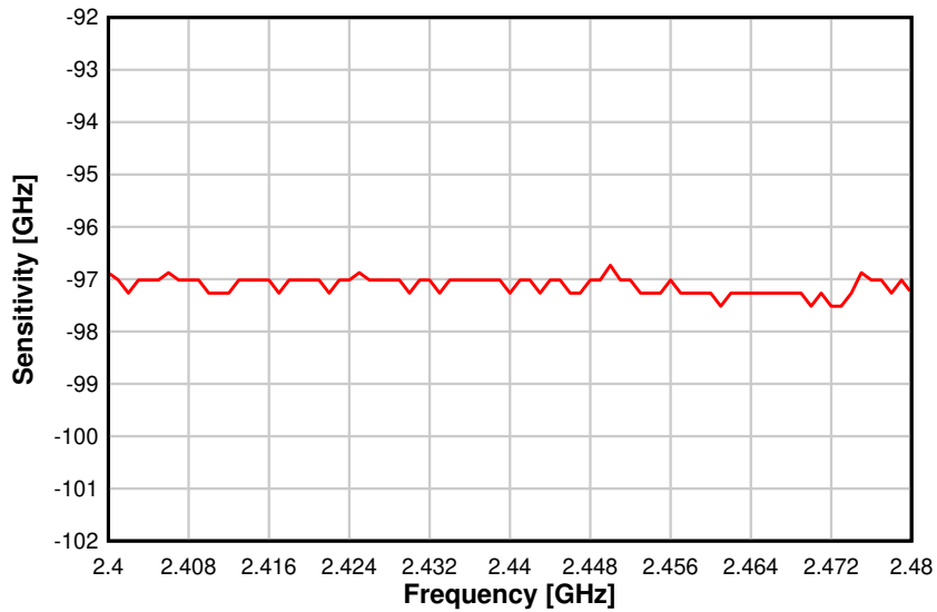
Figure 5-11. Sensitivity vs. Frequency (BLE 1 Mbps, 2.44 GHz)
