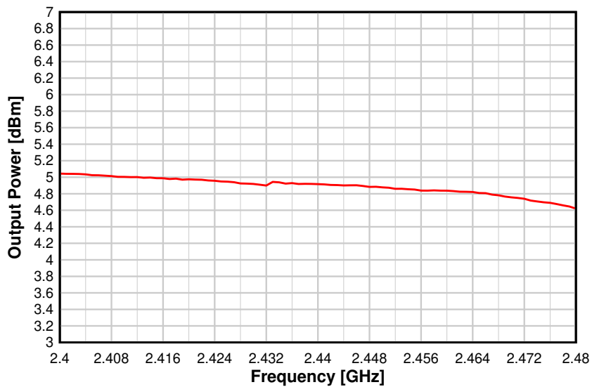
Figure 5-23. Output Power vs. Frequency (BLE 1 Mbps, 2.44 GHz, +5 dBm)
