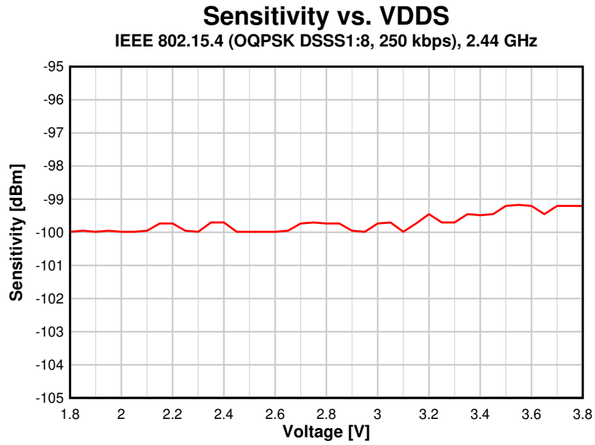
Figure 5-17. Sensitivity vs. Supply Voltage (VDD5) IEEE 802.15.4 (OQPSK DSSS1:8, 250 kbps)
