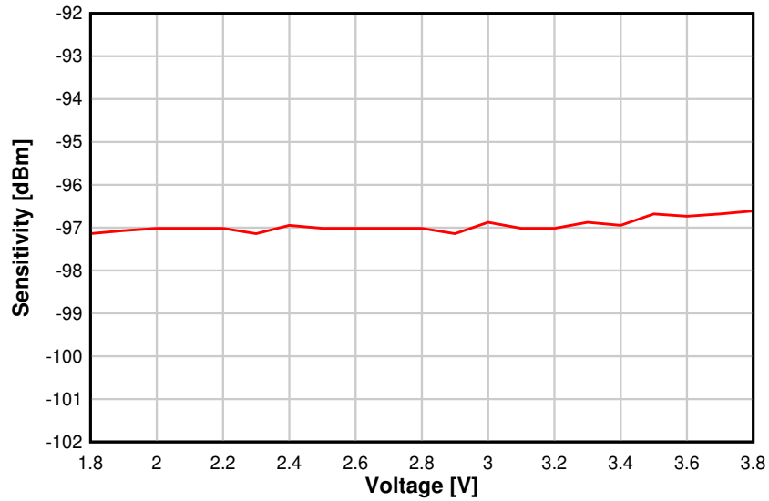
Figure 5-15. Sensitivity vs. Supply Voltage (VDDS) (BLE 1 Mbps, 2.44 GHz)
