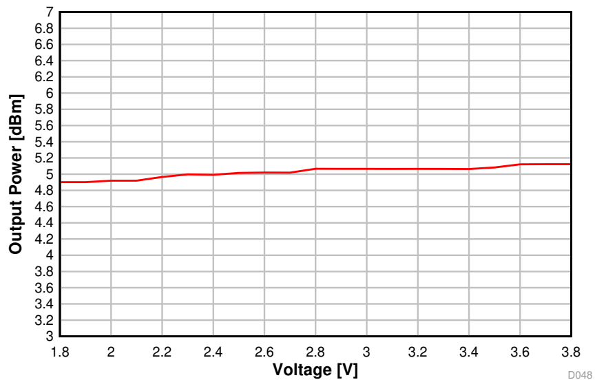
Figure 5-26. Output Power vs. Supply Voltage (VDD5) (BLE 1 Mbps, 2.44 GHz, +5 dBm)
