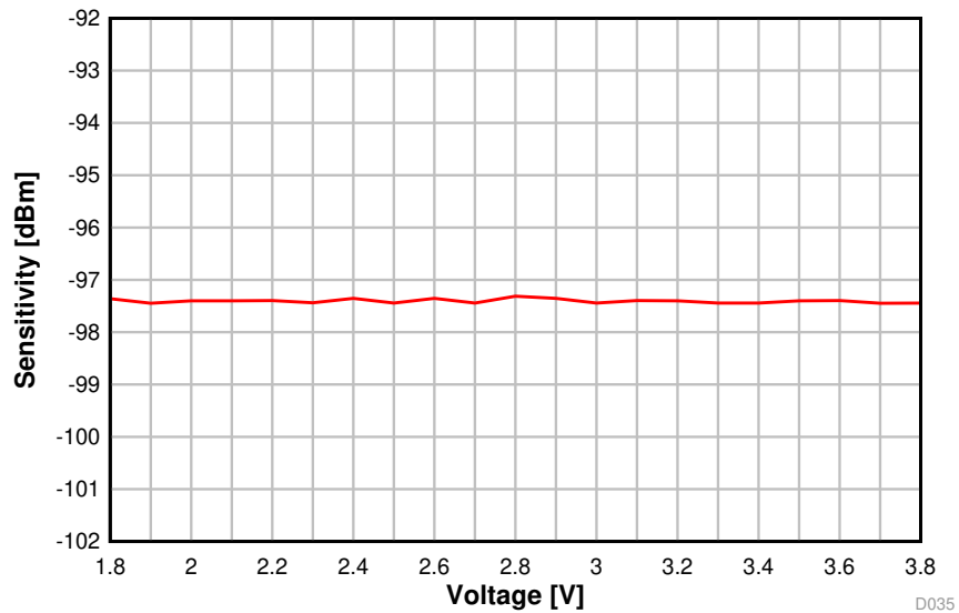
Figure 5-19. Sensitivity vs. Supply Voltage (VDDS) (BLE 1 Mbps, 2.44 GHz, DCDC Off)
