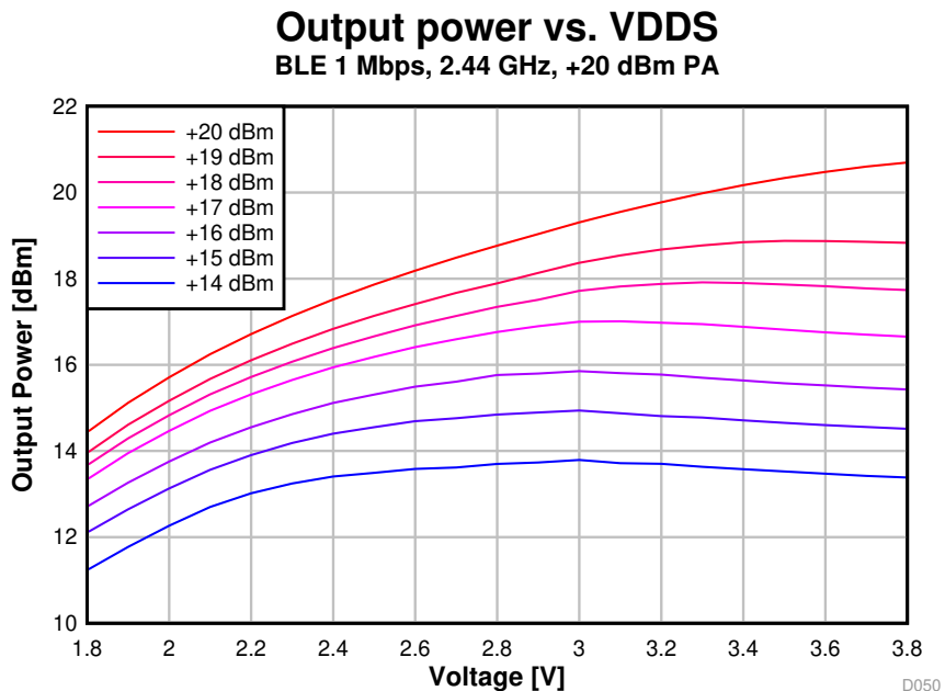
Figure 5-27. Output Power vs. Supply Voltage (VDDS) (BLE 1 Mbps, 2.44 GHz, +20 dBm PA)
