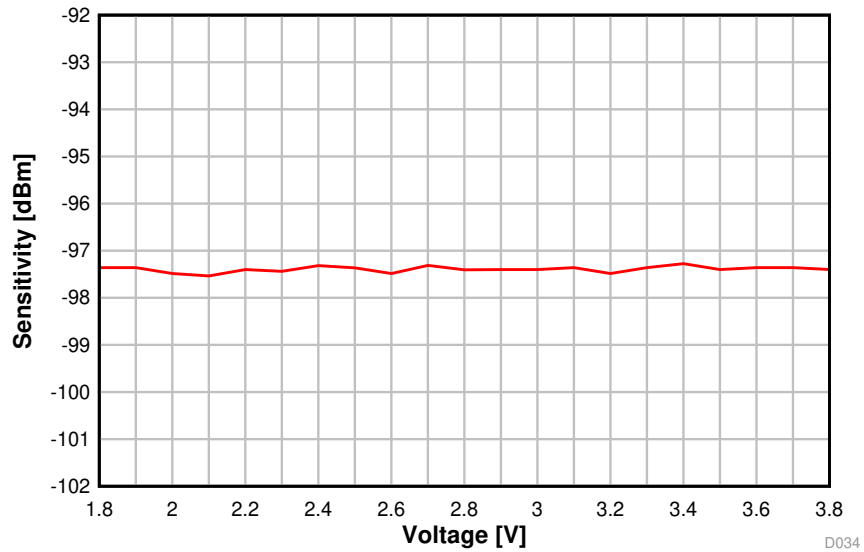
Figure 5-18. Sensitivity vs. Supply Voltage (VDDS) (BLE 1 Mbps, 2.44 GHz)
