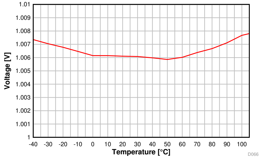
Figure 5-37. ADC Accuracy vs. Temperature
