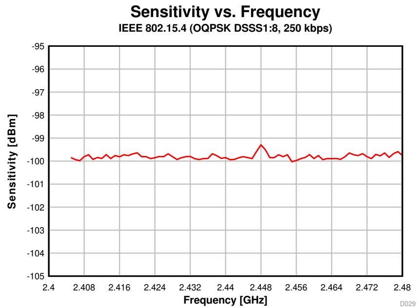
Figure 5-15. Sensitivity vs. Frequency (250 kbps, 2.44 GHz)
