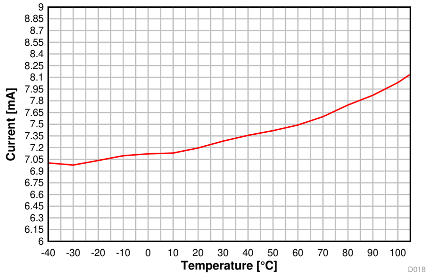
Figure 5-8. TX Current vs. Temperature (BLE 1 Mbps, 2.44 GHz)
