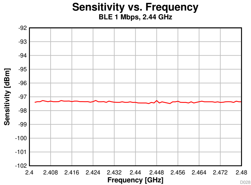
Figure 5-14. Sensitivity vs. Frequency (BLE 1 Mbps, 2.44 GHz)
