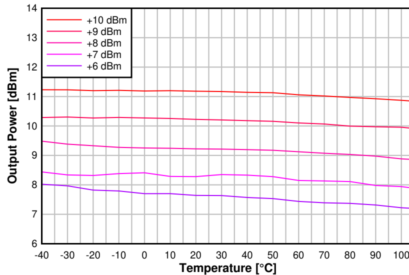
Figure 5-24. Output Power vs. Temperature (2.44 GHz, +10 dBm PA)
