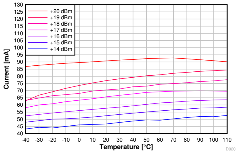
Figure 5-9. TX Current vs. Temperature (BLE 1 Mbps, 2.44 GHz, VDD5 = 3.3 V)
