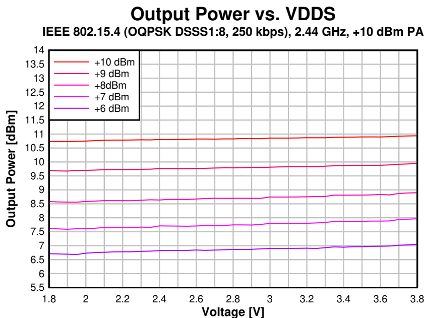
Figure 5-28. Output Power vs. Supply Voltage (VDDS) (2.44 GHz, +10 dBm PA)
