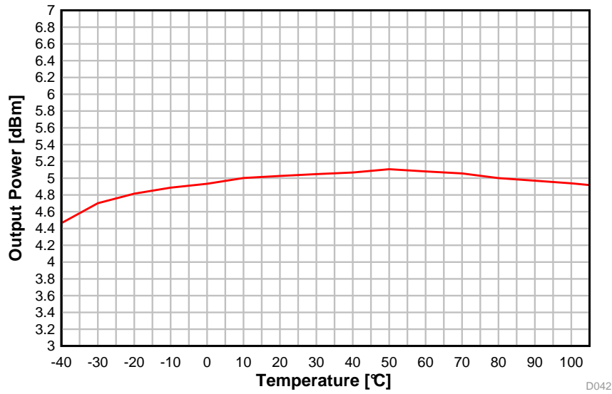
图 5-36. Output Power vs. Temperature (BLE 1 Mbps, 2.44 GHz, +5 dBm)
