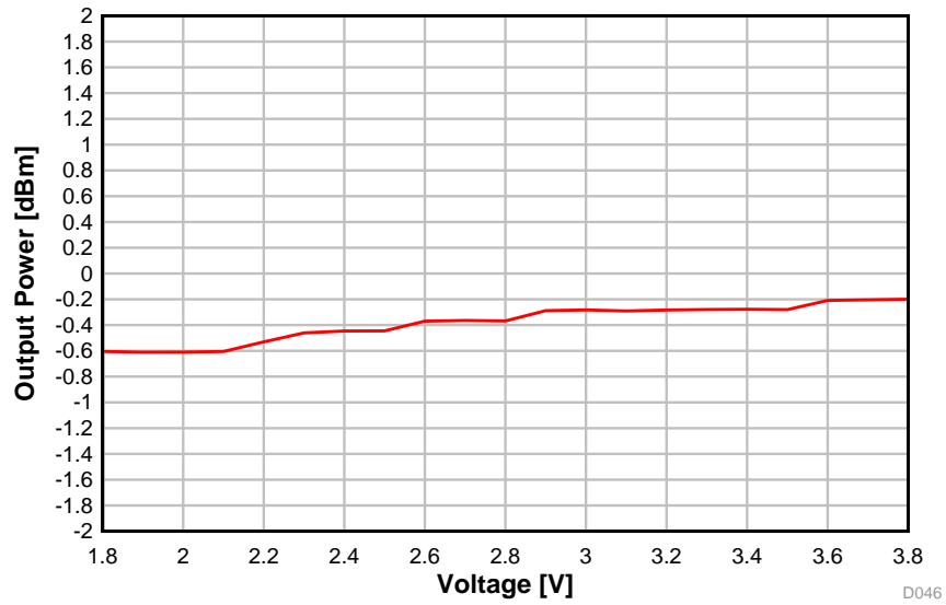
图 5-40. Output Power vs. Supply Voltage (VDD5) (BLE 1 Mbps, 2.44 GHz)
