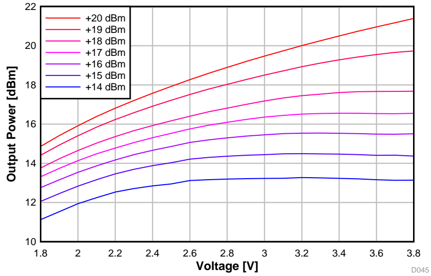
图 5-39. Output Power vs. Supply Voltage (VDD5) (50 kbps, 915 MHz)
