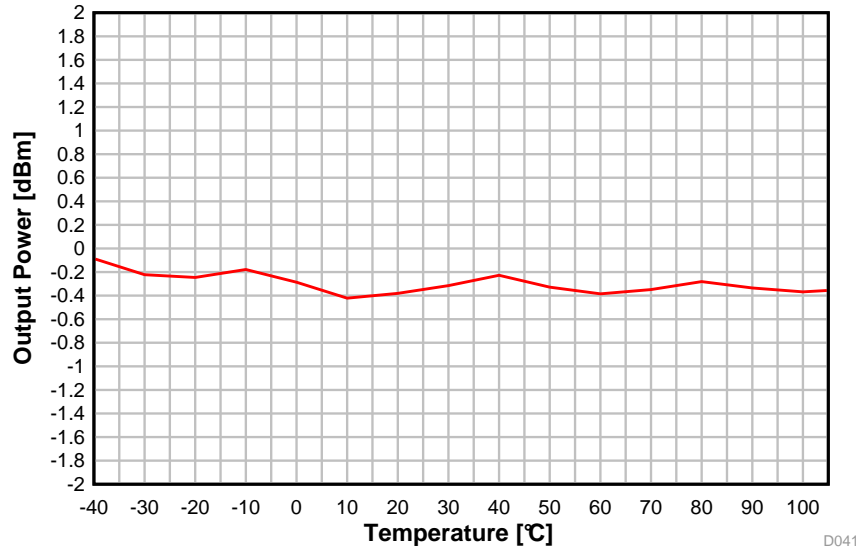
图 5-35. Output Power vs. Temperature (BLE 1 Mbps, 2.44 GHz)
