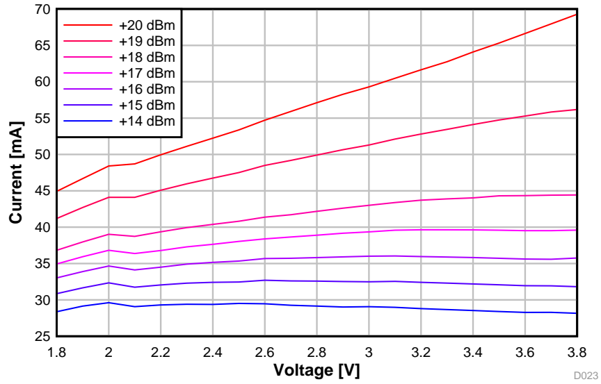
图 5-18. TX Current vs. Supply Voltage (VDDS) (50 kbps, 915 MHz)
