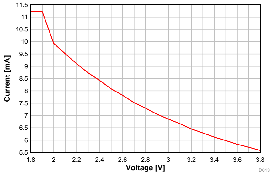
图 5-11. RX Current vs. Supply Voltage (VDD5) (BLE 1 Mbps, 2.44 GHz)
