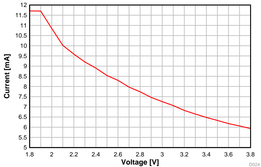
图 5-19. TX Current vs. Supply Voltage (VDDS) (BLE 1 Mbps, 2.44 GHz)
