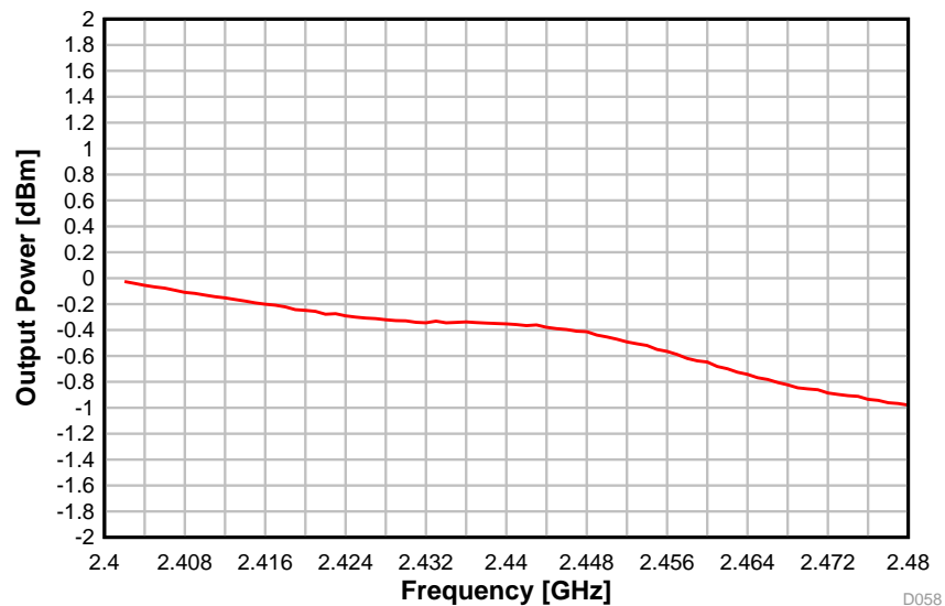
图 5-46. Output Power vs. Frequency (BLE 1 Mbps, 2.44 GHz)
