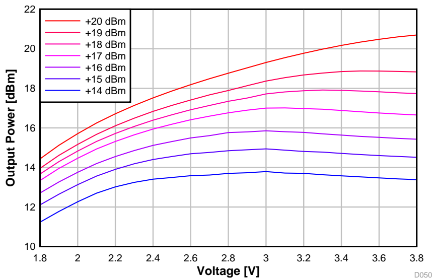
图 5-42. Output Power vs. Supply Voltage (VDD5) (BLE 1 Mbps, 2.44 GHz, +20 dBm PA)
