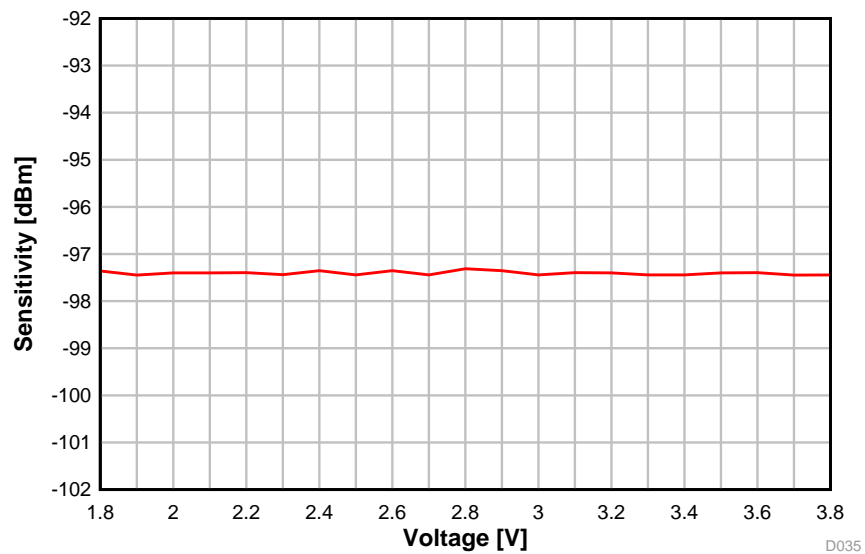
图 5-30. Sensitivity vs. Supply Voltage (VDDS) (BLE 1 Mbps, 2.44 GHz, DCDC Off)
