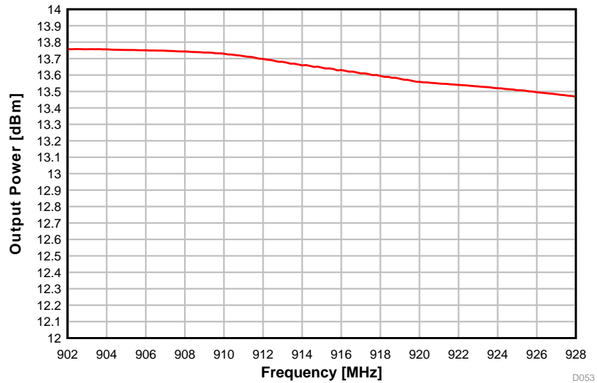
图 5-44. Output Power vs. Frequency (50 kbps, 915 MHz)
