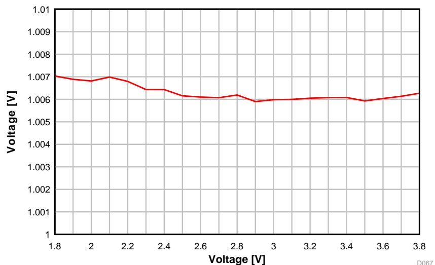
图 5-54. ADC Accuracy vs. Supply Voltage (VDD5)
