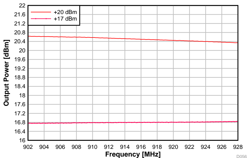
图 5-45. Output Power vs. Frequency (50 kbps, 915 MHz, VDDS = 3.3 V)
