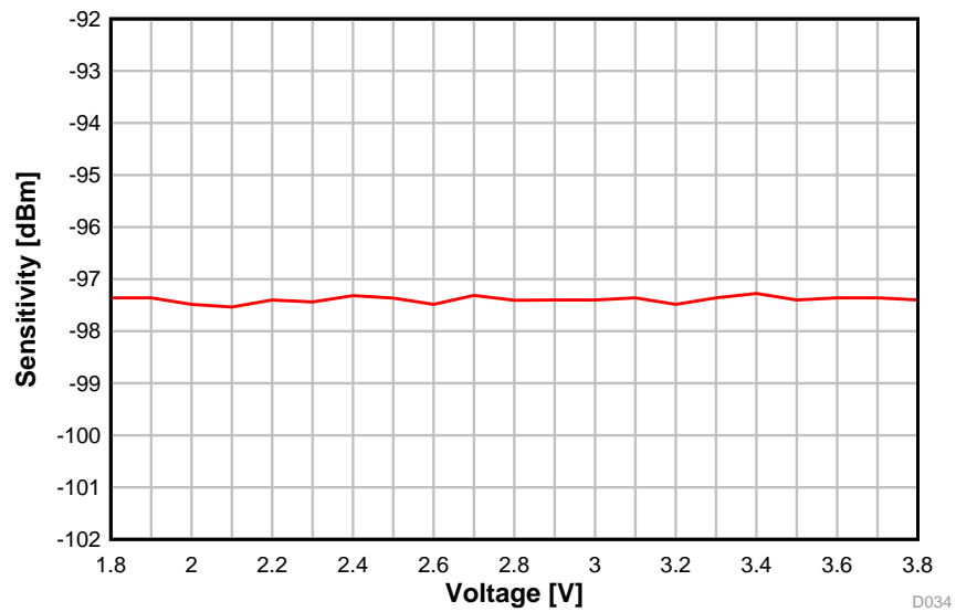
图 5-29. Sensitivity vs. Supply Voltage (VDDS) (BLE 1 Mbps, 2.44 GHz)
