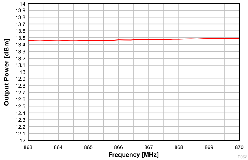
图 5-43. Output Power vs. Frequency (50 kbps, 868 MHz)
