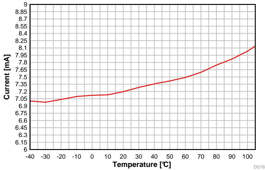
图 5-15. TX Current vs. Temperature (BLE 1 Mbps, 2.44 GHz)
