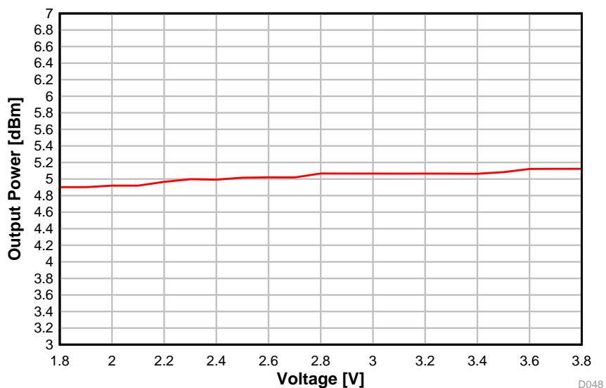
图 5-41. Output Power vs. Supply Voltage (VDD5) (BLE 1 Mbps, 2.44 GHz, +5 dBm)
