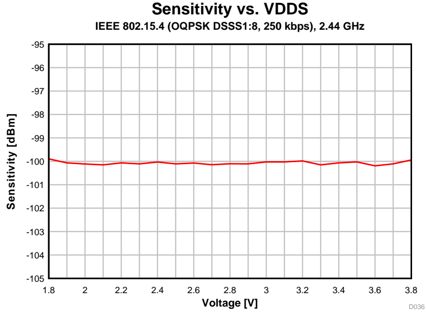
图 5-31. Sensitivity vs. Supply Voltage (VDD5) (250 kbps, 2.44 GHz)
