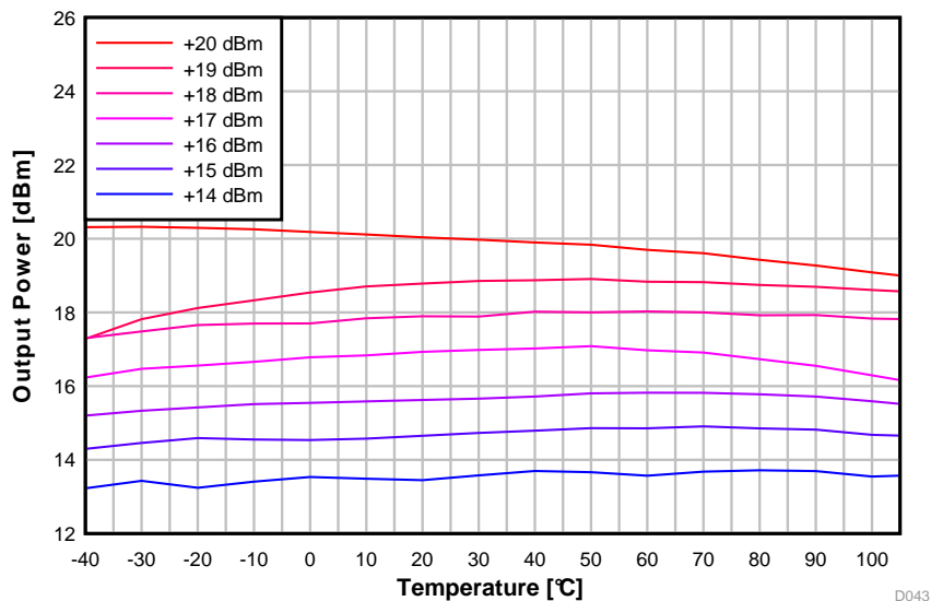
Output Power vs. Temperature BLE 1 Mbps, 2.44 GHz, +20 dBm PA, VDD5 = 3.3 V
