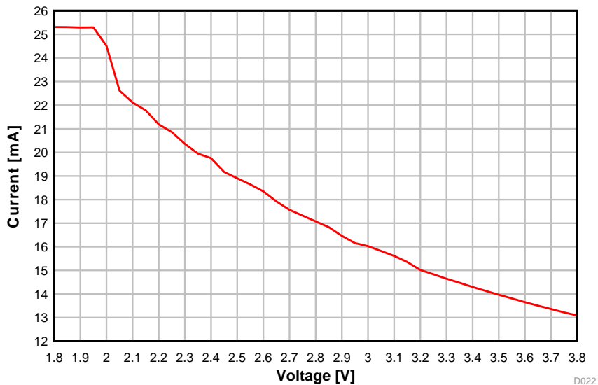
图 5-17. TX Current vs. Supply Voltage (VDD5) (50 kbps, 868.3 MHz)
