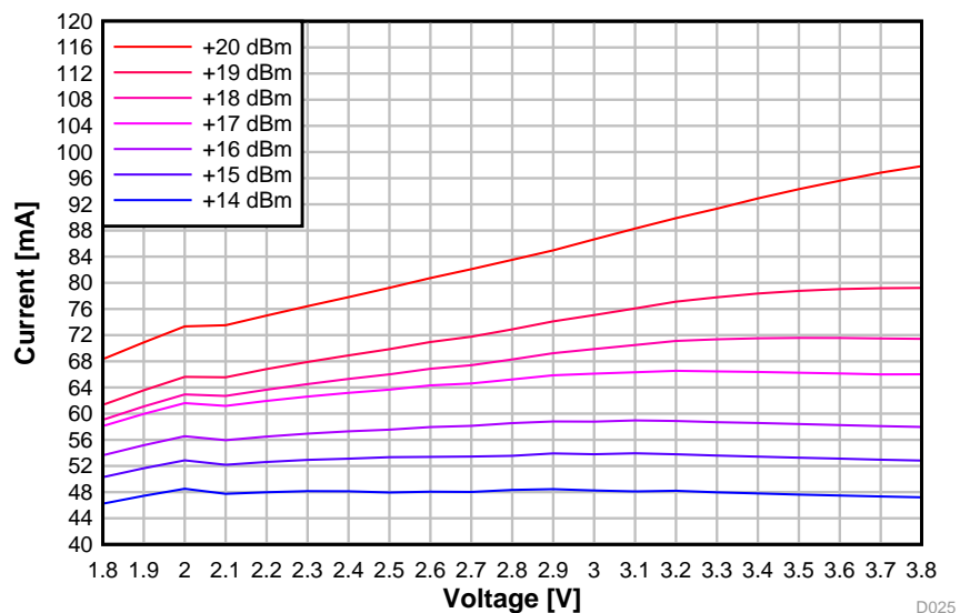
图 5-20. TX Current vs. Supply Voltage (VDD5) (BLE 1 Mbps, 2.44 GHz, +20 dBm PA)
